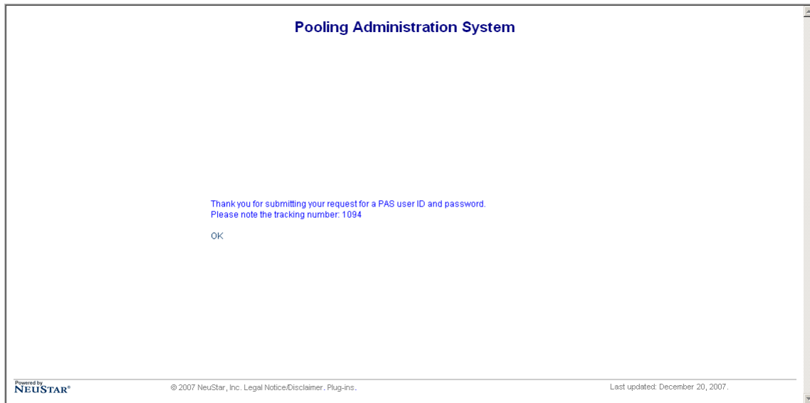
Figure 5 - Confirmation Screen
